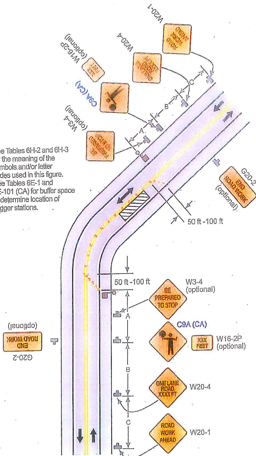
Typical Application 10
